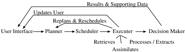
Figure 1: BIG's Problem Solving Control Flow
